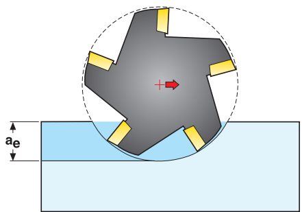
Side milling
