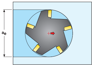
Slot milling
