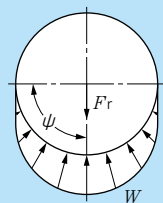
Fig. 3.10 \varepsilon = 0.5 \psi = \pm 90^\circ Radial clearance 0
