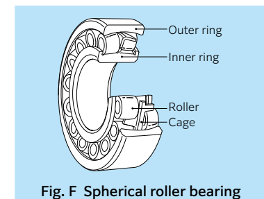
Fig. F Spherical roller bearing
