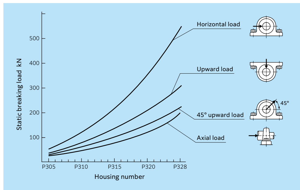
Fig. 3 Static breaking load of P3 type
