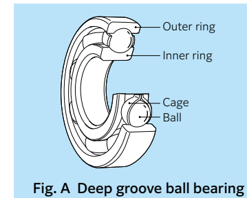
Fig. A Deep groove ball bearing
