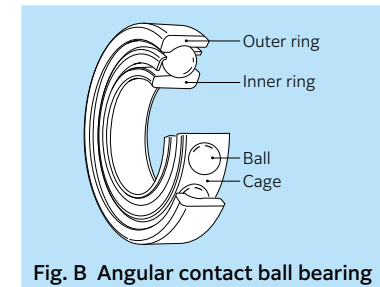
Fig. B Angular contact ball bearing
