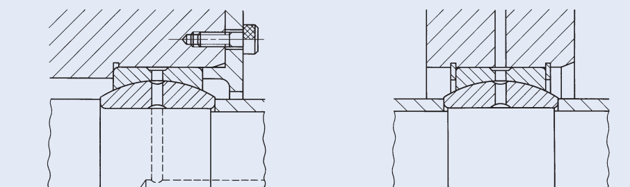
Fig.10 Mounting examples
