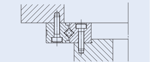
Fig.2 Mounting example -1 Mounting Holed Type High Rigidity Crossed Roller Bearing
