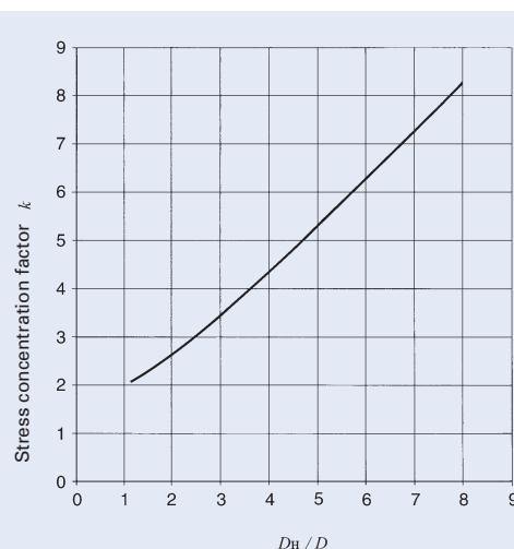
Fig.7 Stress concentration factor
