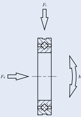
Fig. 1 Load direction
