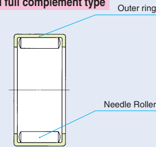
Grease retained full complement type
