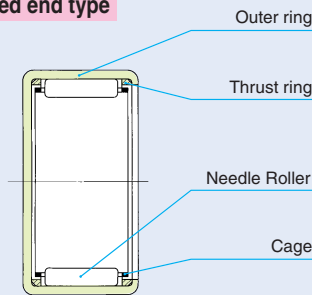
Caged and closed end type
