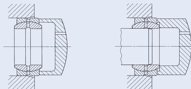
Fig.9 Mounting method
