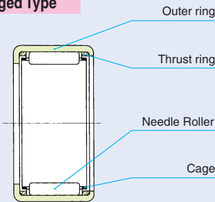
Standard Caged Type
