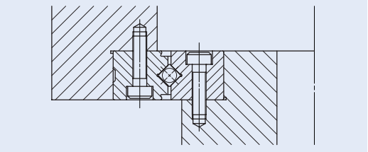
Fig.3 Mounting example -2 Mounting Holed Type High Rigidity Crossed Roller Bearing
